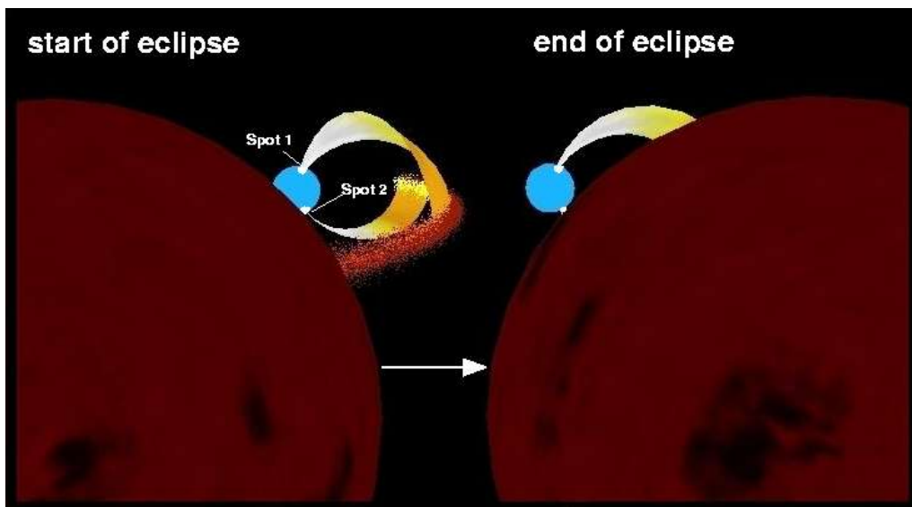
Figure 2. Earth Observer' s View Of A Polar At The Start (Left) and End (Right) Of Eclipse.
