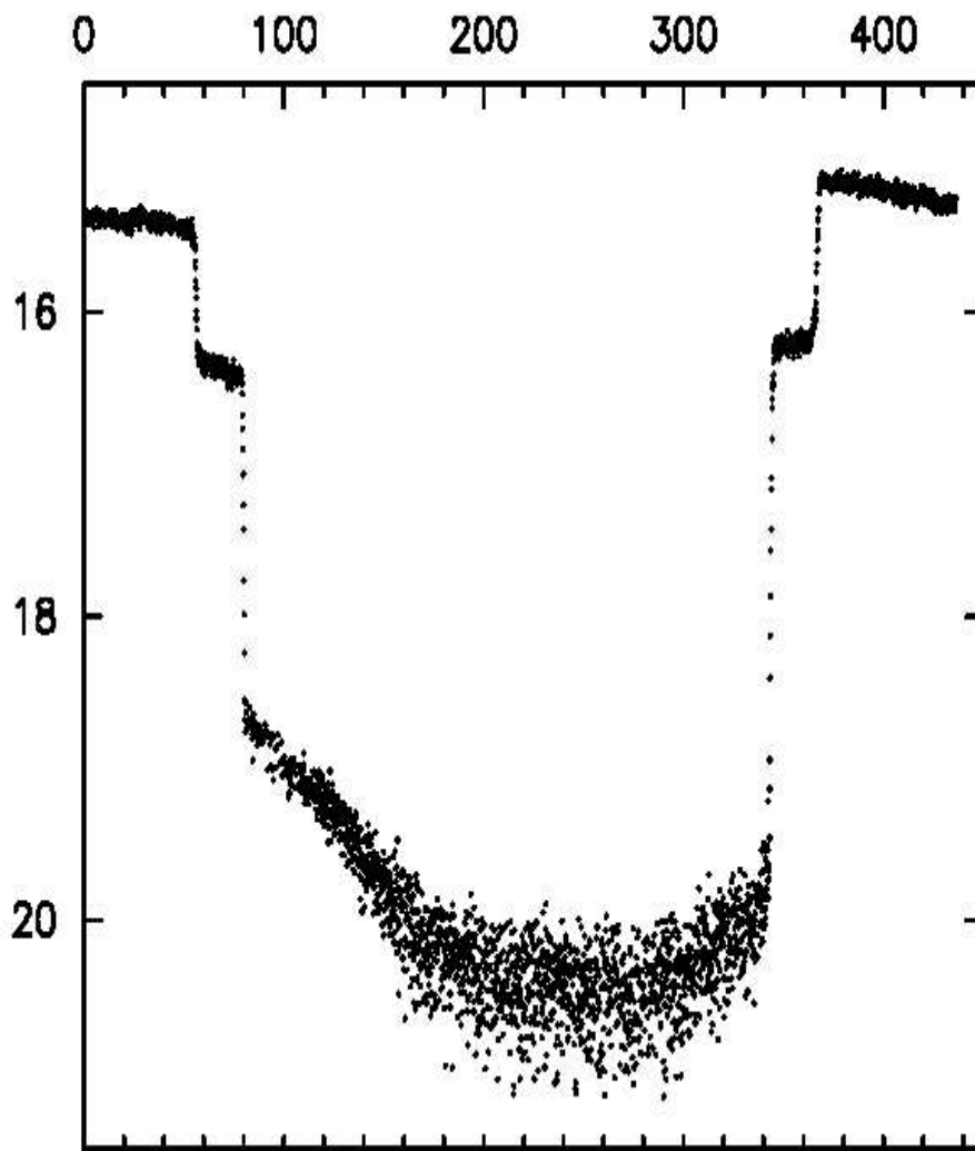
Figure 3. Sequence of brightness measurements of the polar. Each point is a 112 millisecond exposure.
