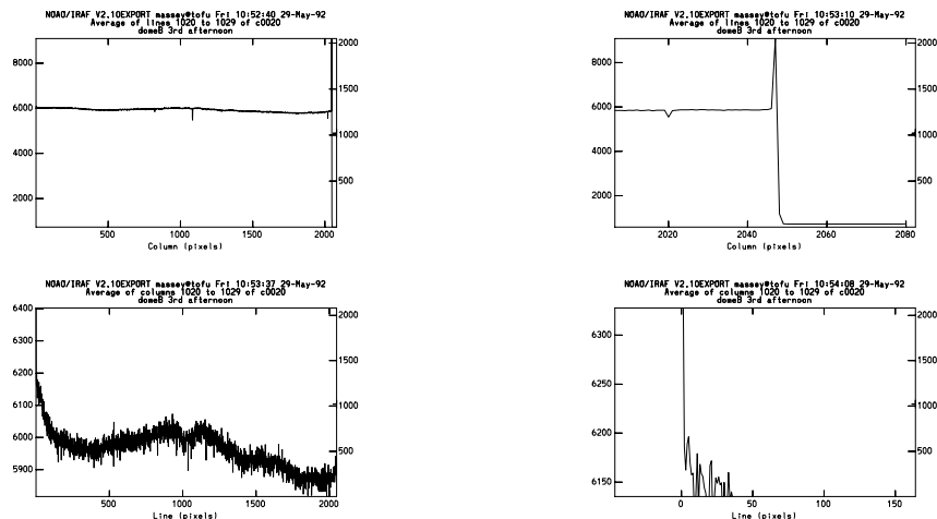
Figure 25: The bias and trim parameters in the header are confirmed to be reasonable by implotting a dome-flat exposure.
