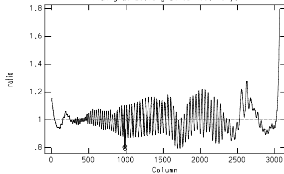
Figure 12: The top plot shows the fit of an order=1 cubic spline on the flat-field data. The middle plot shows an order=6 fit obtained by typing a :order 6 followed by an f . The bottom plot shows the ratio of the data to the fit, which can be viewed by hitting the j key. An h brings back the data vs. pixel number plot. For more information do a help icfit .
