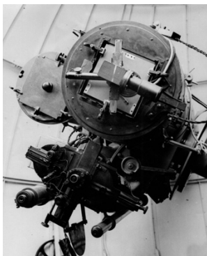
Fig 11. The first Cape photometer when mounted on the 13-inch Astrographic telescope (SAAO Archives P2964).
