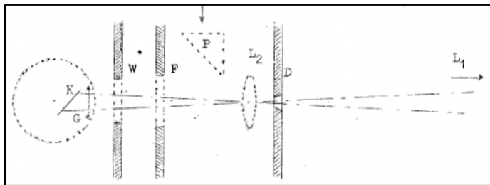
Fig 12. Optical diagram of the first photometer. Starlight entered from the right through the focal plane aperture D and the exit pupil of the telescope was focused by the lens L2 onto the photocathode of the photomultiplier K after passing through the filter F. A retractable prism P was used for
