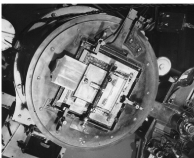
Fig 4. Fabry photometer mounted in place of a plateholder at the focus of the 13-inch refractor. The removable plateholder and dark slide was adjusted in position between exposures. The filter, Fabry lens and aperture were below the plateholder (Cousins, Thesis).
