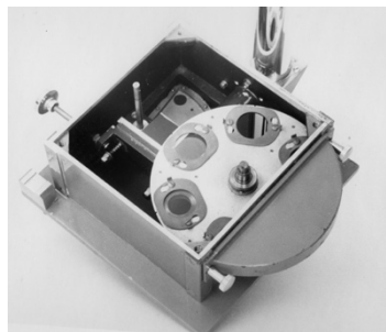
Figs 22 & 23. The Cousins photometer (2 nd type, end-window version) shown with and without the filter wheel in place. It was clearly very similar to the first version (see Fig 18) (SAAO Photos: P7577, P7578).
