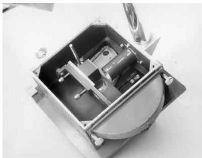
Figs 22 & 23. The Cousins photometer (2 nd type, end-window version) shown with and without the filter wheel in place. It was clearly very similar to the first version (see Fig 18) (SAAO Photos: P7577, P7578).
