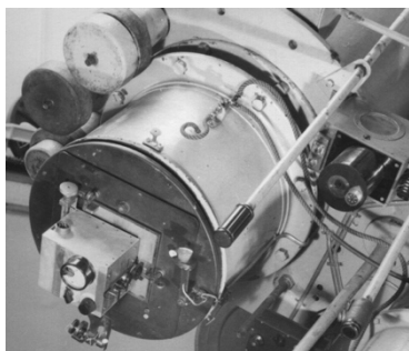
Fig 28. The photometer in this photograph is believed to have been that used for occultation observations by Cousins & Guelke (1953). It no longer exists. Shown here attached to the McClean 24-inch refractor. The early voltage divider (Fig 13) can also be seen. (SAAO Photo: P5655).
