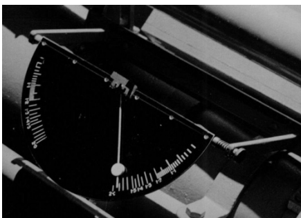
Fig 8. Cousins Airmass Indicator. The axis was mounted parallel to the tube of the telescope and the scale stayed in a vertical plane (SAAO Archives P3571).
