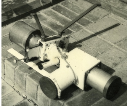
Fig 26. The Leiden photometer supplied to the Radcliffe Observatory. It was attached to the Observatory's prism spectrograph in place of its large "Visitors' eyepiece". The latter was then inserted into the side of the photometer as a field acquisition eyepiece. At the time this photograph was taken, a Cousins-type photomultiplier housing for an EMI tube had already been substituted for the original 931A type and braces had been added to reduce flexure. (Photo: ISG, private collection)
