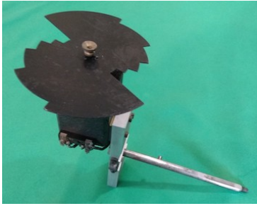
Fig 3. Rotating sector with \frac{1}{2} mag steps. It could be inserted quickly near the optical axis of the telescope and positioned for a particular step by a lever. SAAO Museum Inv. M046, part (photo: ISG)
