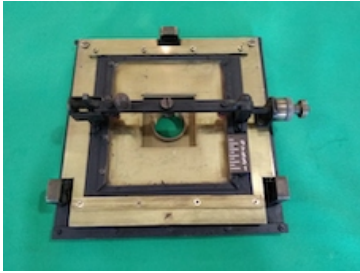
Fig 5. Fabry photometer baseplate without plateholder. The filter, Fabry lens and aperture screwed into the central hole. SAAO Museum Inv. M046, part (Photo: ISG)
