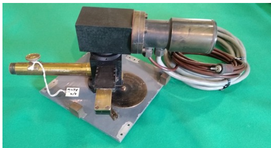
Fig 10. First Cape photoelectric photometer as it exists today and (below, Fig 11) when mounted on the 13-inch Astrographic telescope. SAAO Museum Inv. M098/4 (Photo: ISG).
