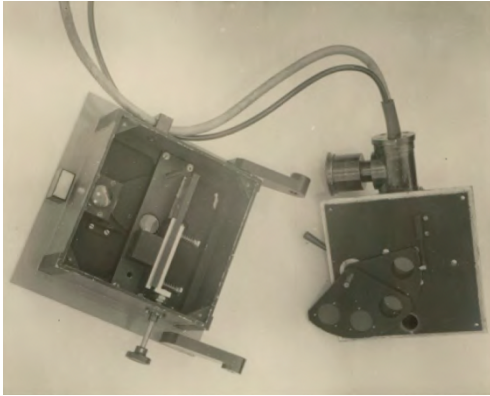
Fig 18. Cousins's second photometer in its original form, shown with the top removed. It contained the same elements as the earlier one but was more rigid and easier to use. The part on the right that has the 931A photomultiplier attached is still in existence but the base was used as part of the later version with an E.M.I. end-window tube. Attached to the side of the phototube enclosure was a container with dessicant. The base of this instrument was hinged so that it could be swung out, possibly so that a wider-field eyepiece could be used for finding purposes (From Cousins, Thesis, 1953).
