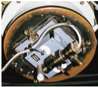
Fig 19. The second photometer on the Astrographic telescope around January 1962. It is surprising that it was still in use at this date in view of the superior performance of the EMI end-window tubes. (Photo: Greg Roberts).
